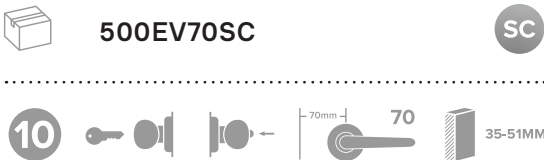
Empire Entrance Lock Leverset – EV Series 70mm Backset
